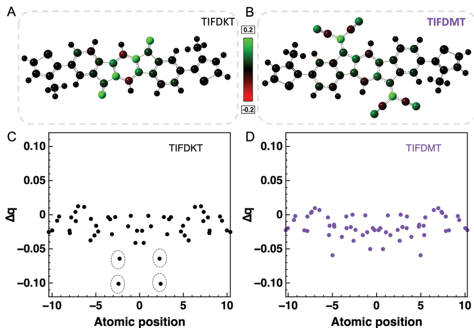
Figure 4. DFT-calculated electronic spin densities in n-doped TIFDKT (A) and TIFDMT (B) molecules, and the corresponding Mulliken charge distributions (C and D, respectively, dash circles highlight undesirable charge localization in TIFDKT).
